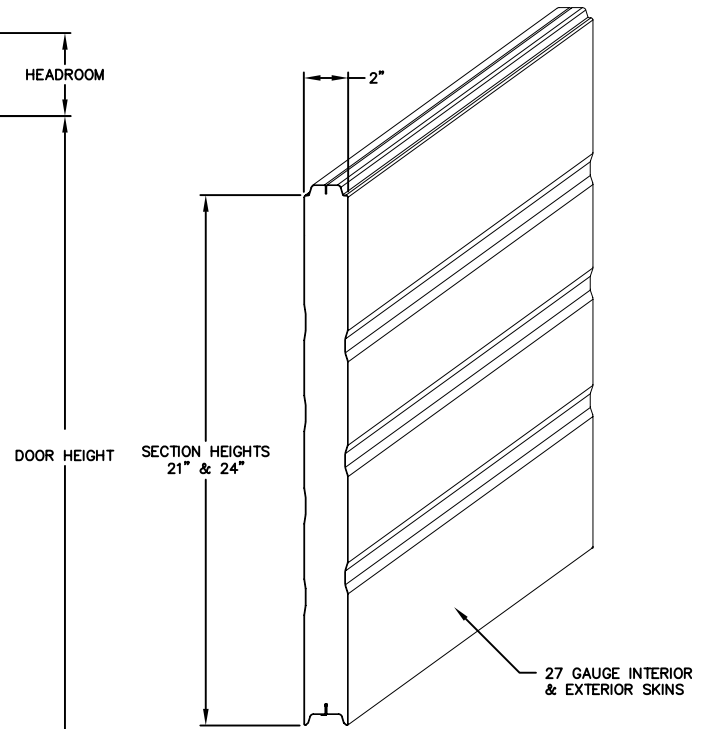
ISOMETRIC PROFILE
