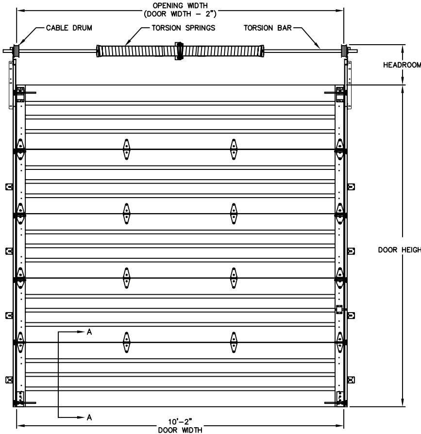
INTERIOR ELEVATION
